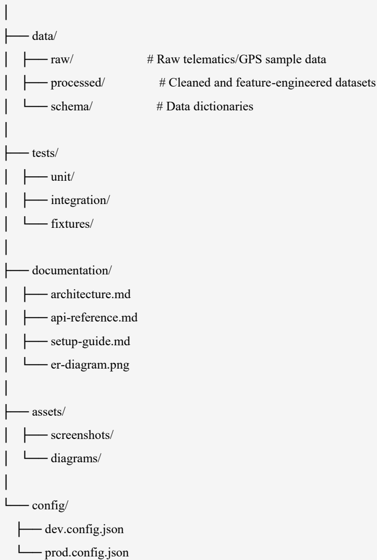
Figure 2.1 — Recommended repository structure for the Smart Fleet Analytics Platform
